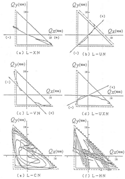
Figure 12 The Lateral Loads Q_x and Q_y .
