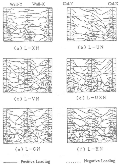
Figure 5 Cracking Patterns.
