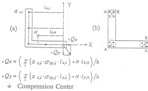
Figure 10 Calculation Method for Bi-Directional Bending Strength.
