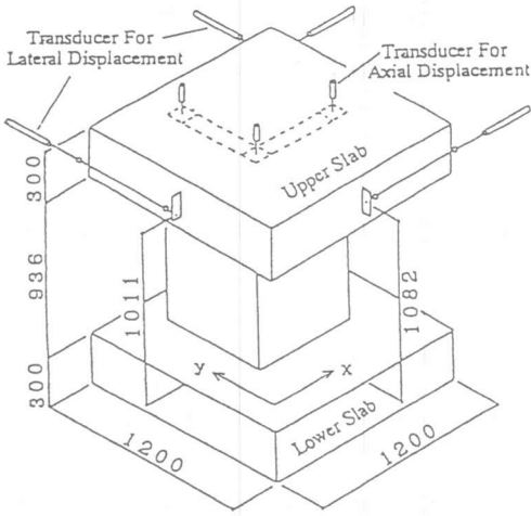
Figure 1 Details of Specimens (mm).
