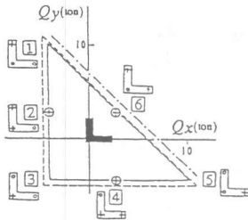
Figure 11 Bi-Directional Bending Strength Diagram.
