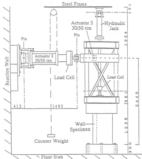
Figure 4 Loading Apparatus (mm).
