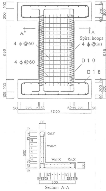
Figure 2 Details of Reinforcement.
