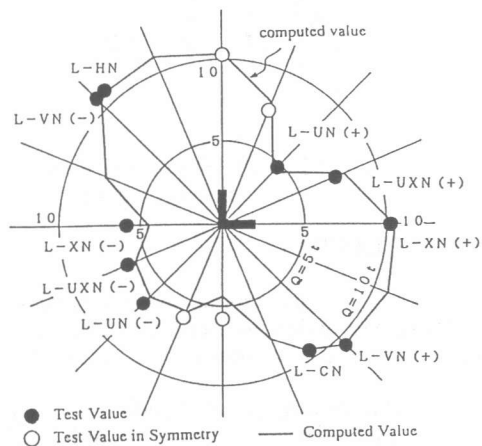
Figure 9 Bending Strength Diagram in Deflection Direction.
