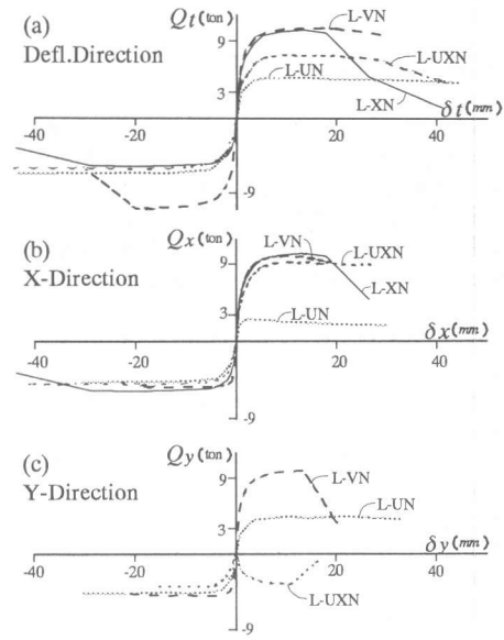
Figure 6 Max. Load-Deflection Curves at Each Cycle.
