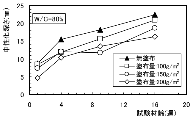
図-9 中性化深さの経時変化(W/C=80%)
