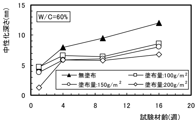
図-8 中性化深さの経時変化(W/C=60%)
