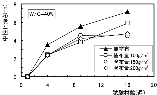
図-7 中性化深さの経時変化(W/C=40%)
